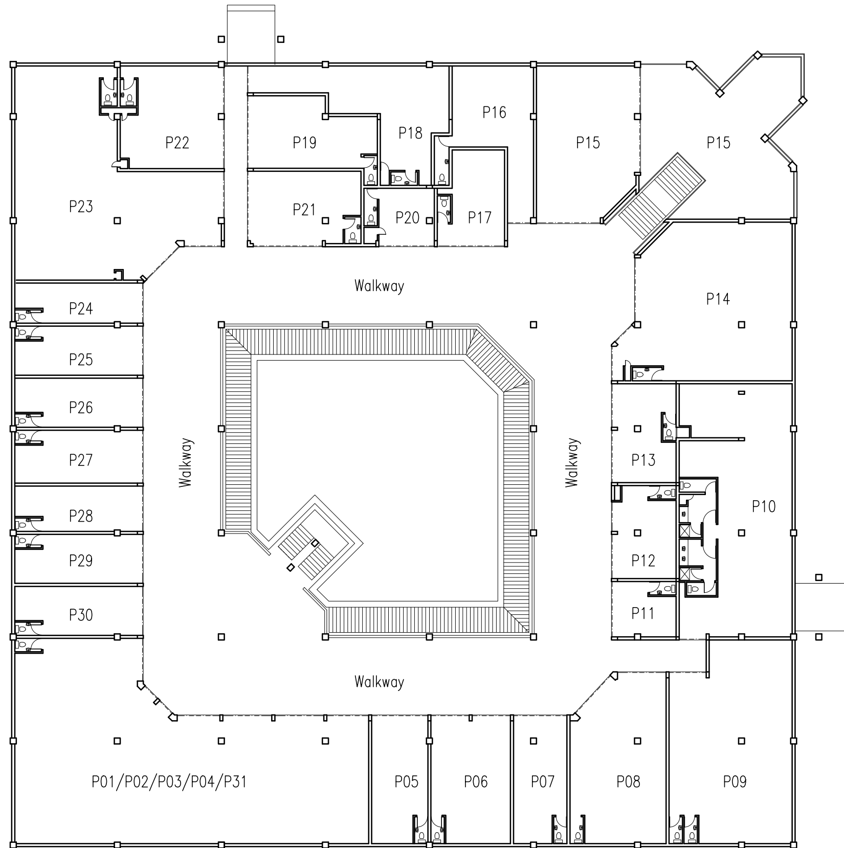
First floor plan Scale :- 1 : 250
